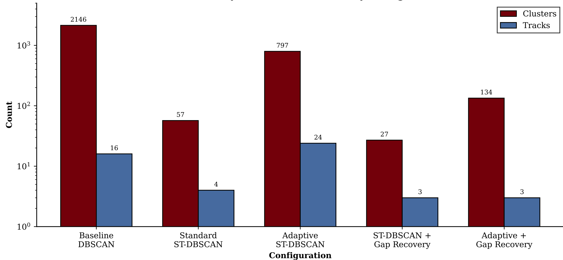
Ablation Study: Clusters and Tracks by Configuration
